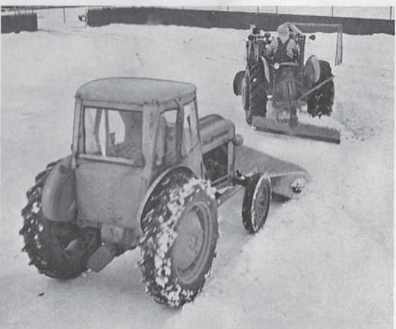
Ice rinks —Blade and broom make an efficient tandem team for quick clean-up between skating sessions. Tractor-loader also dumps excess snow, tows planer.
